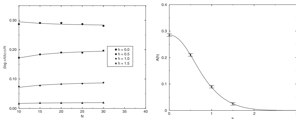
Figure 3. Numbers of metastable states. \log \langle N(h) \rangle / N versus N at different magnetic fields, see legend (left). Data points show the field dependence of A_{ROM}(h) obtained from the fits, while the full curve indicates the analytical results in the thermodynamic limit (right).
