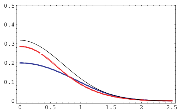
Figure 4. A_{SK}(h) (bottom), A_{ROM}(h) (middle) and \frac{1}{\pi} e^{-h^2} (top). (This figure is in colour only in the electronic version)
