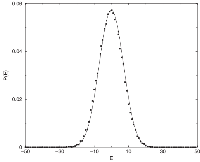
Figure 1. Probability distribution function P_{\text{ROM}}(E) for the ROM model (full curve). Simulation for a N = 100 ROM (data points). For a fixed spin configuration, 10^6 realizations of disorder were generated.
