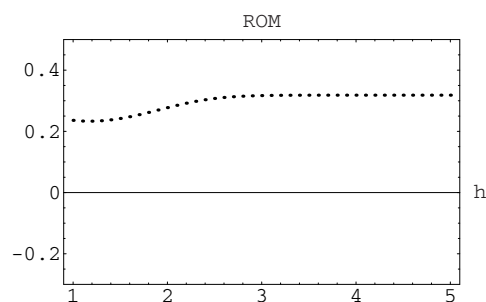
Figure 5. Plot of e^{h^2} A_{ROM}(h) for values of the magnetic field h between 1 and 5.
